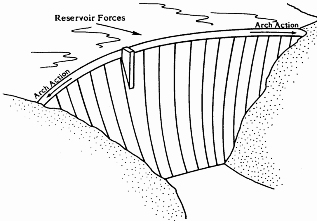
FIGURE I-3. SIMPLIFIED VIEW OF AN ARCH DAM
