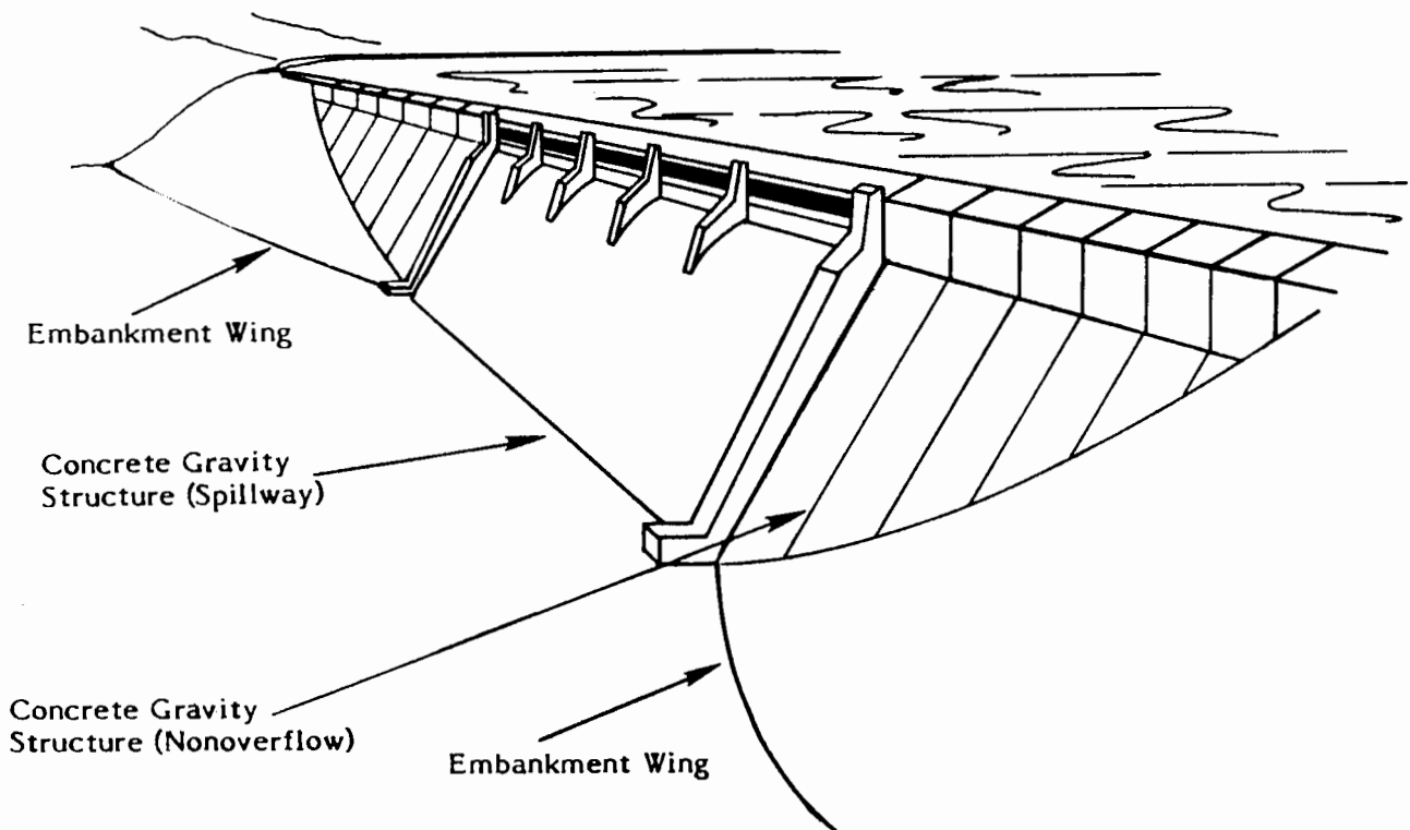
FIGURE I-4. COMPOSITE DAM
