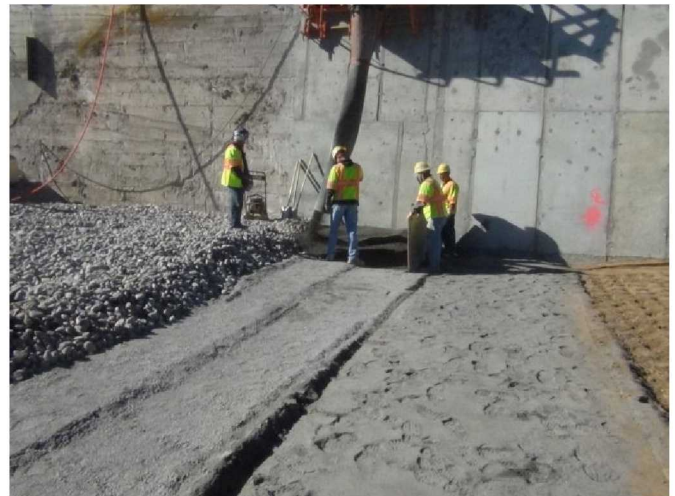
Photo 1. Placement of a 3-stage filter showing use of hand-held plywood shield to limit cross contamination.
