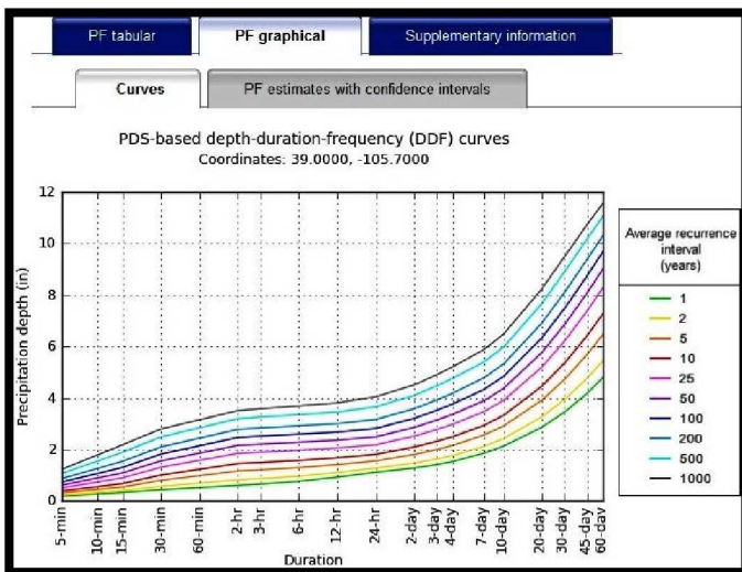
Figure 6: Graphical Precipitation Frequency Curves
