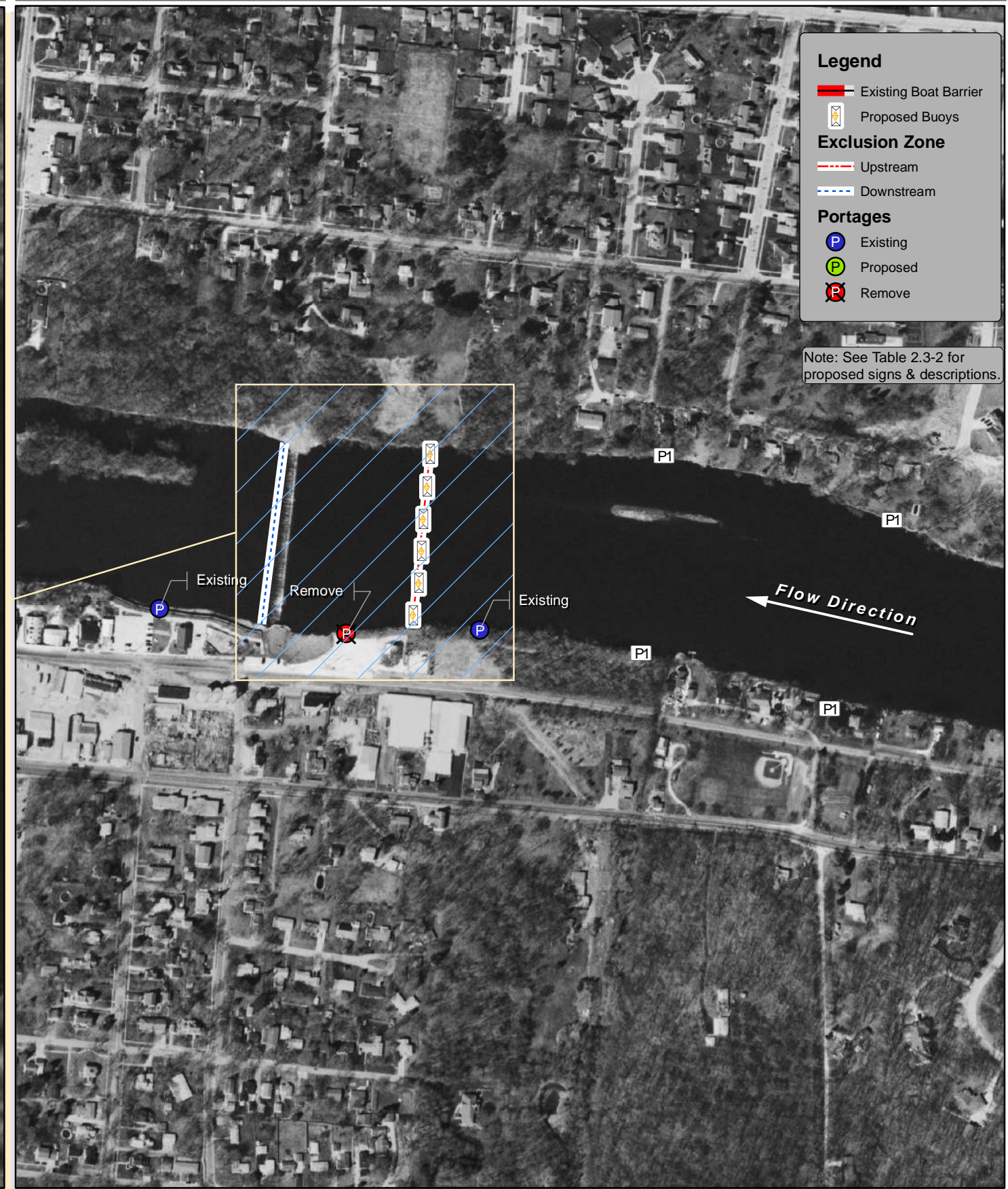
Yorkville Dam - Fox River Yorkville, Illinois
