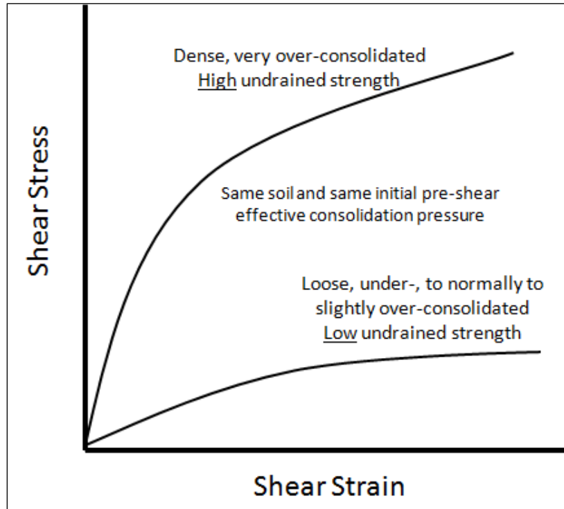
Figure IV-3-1. Typical Undrained Stress Strain Curves for Loose and Dense Soils.
