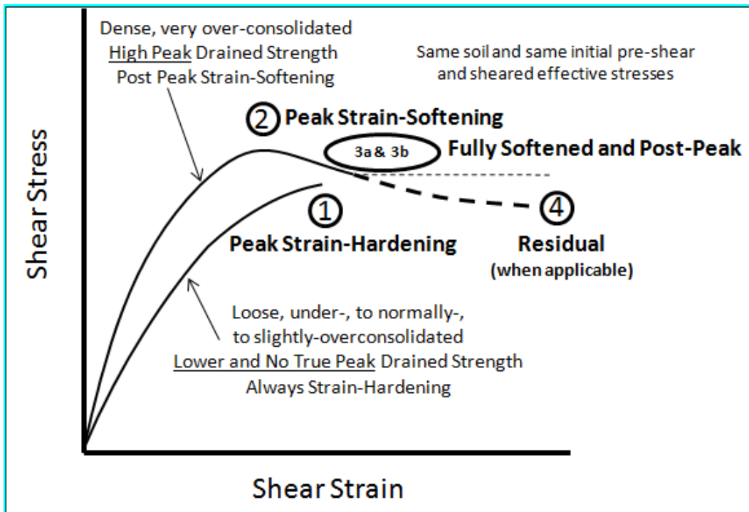
Figure IV-3-2. Generalized Drained Stress Strain Curves for Loose and Dense Soils and Types of Strengths Considered for Use in Stability Analyses.
