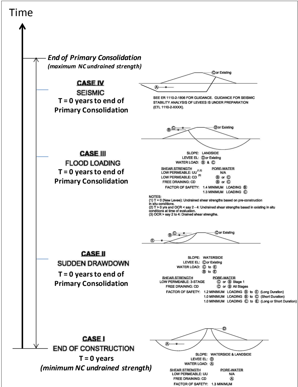
Figure IV-3-3. Example Slope Stability Loading Conditions and Typical Associated Design Factors of Safety for Levee Evaluations. Similar Conditions Apply to Dams.
