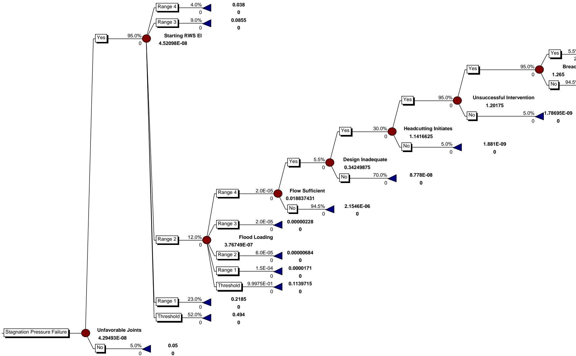
Figure F-1-3 – Example Event Tree
