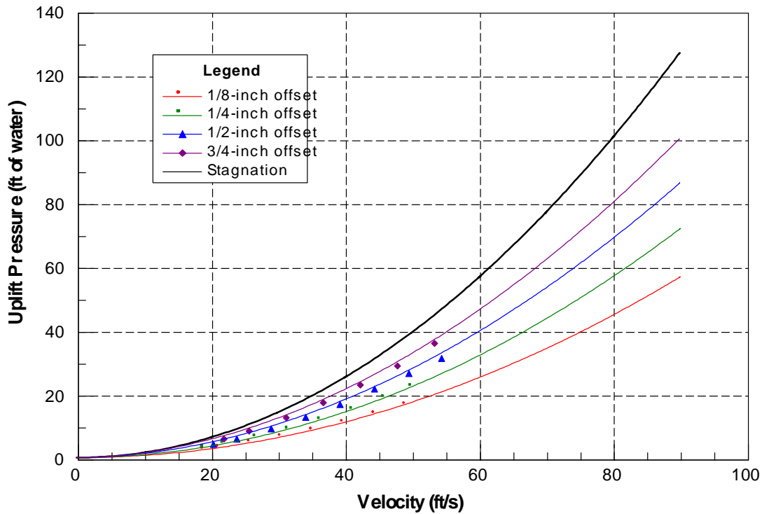
Figure F-1-4 - Mean uplift pressure, sharp-edged geometry, sealed cavity, 1/8-inch gap.
