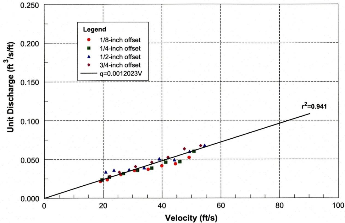
Figure F-1-8 – Unit discharge for joint/crack, sharp-edged geometry, 1/2-inch gap.
