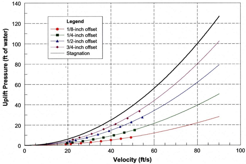
Figure F-1-6 – Mean uplift pressure, sharp-edged geometry, vented cavity, 1/2-inch gap.
