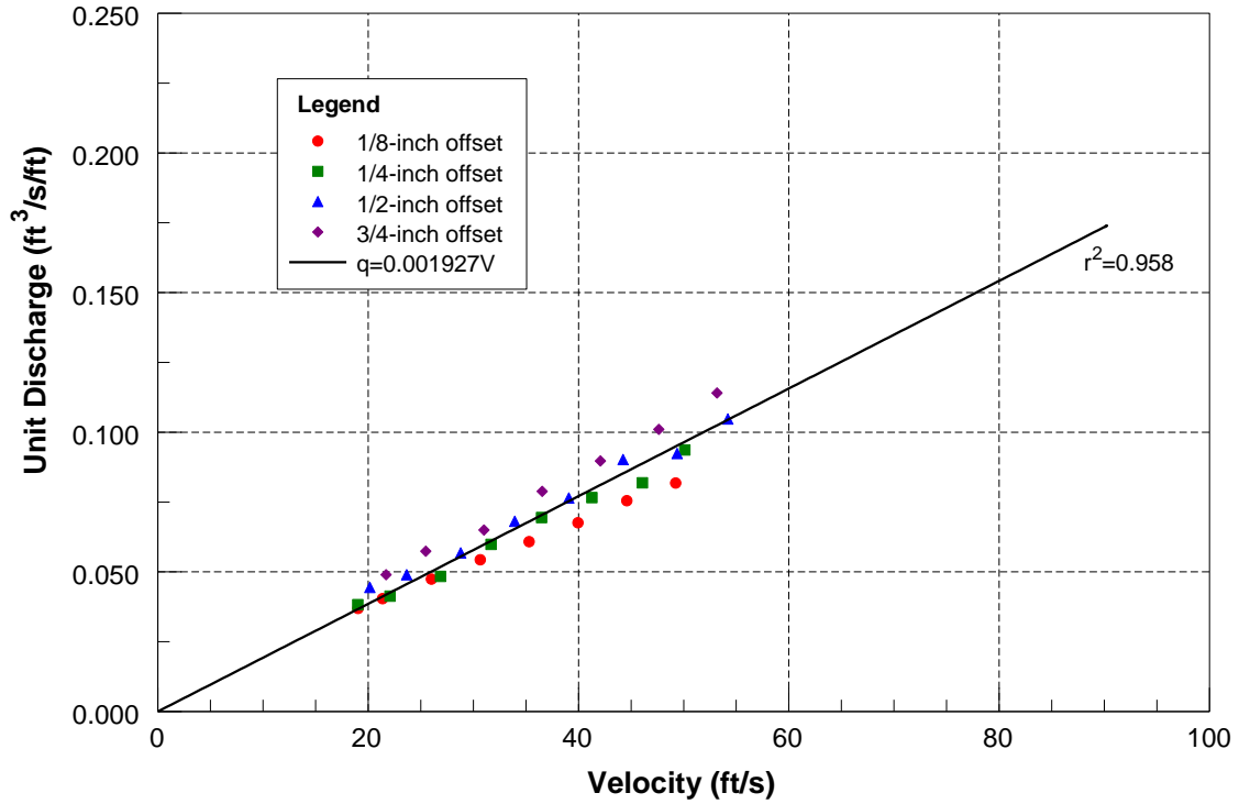
Figure F-1-7 – Unit discharge for joint/crack, sharp-edged geometry, 1/8-inch gap.
