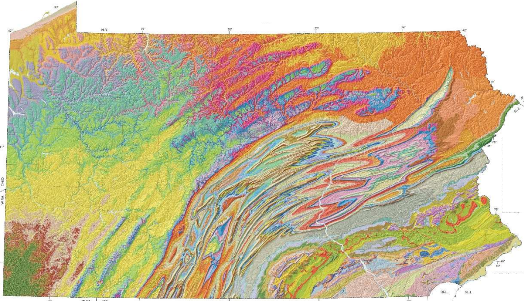
Figure 1: Geology of Pennsylvania. The Appalachian Mountains are shown as multicolored lines running through the center of the state. The Allegheny Mountains divide this zone from the Appalachian Plateau, shown in yellow. Source: Miles (2008).
